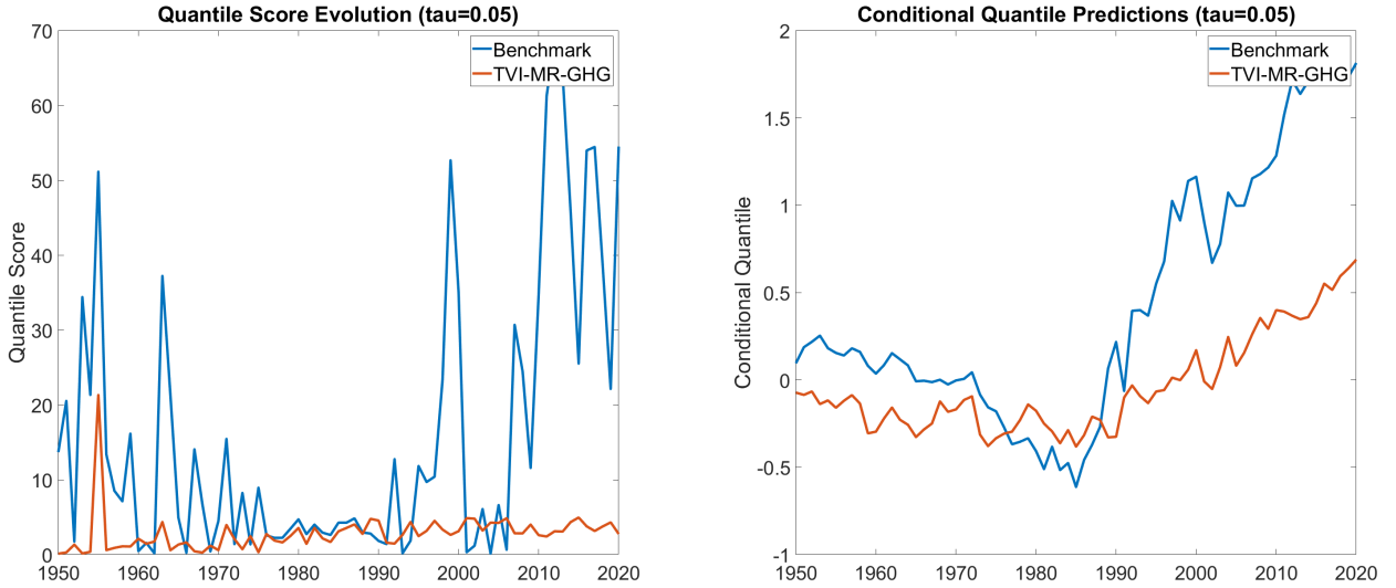
Figure 5: Quantile Score evolution (left panel) and the predicted conditional quantile (right panel) for the 5 th conditional quantile of global temperatures for specific models.
