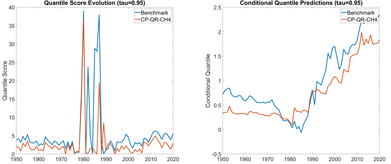
Figure 6: Quantile Score evolution (left panel) and the predicted conditional quantile (right panel) for the 95 th conditional quantile of global temperatures for specific models.
