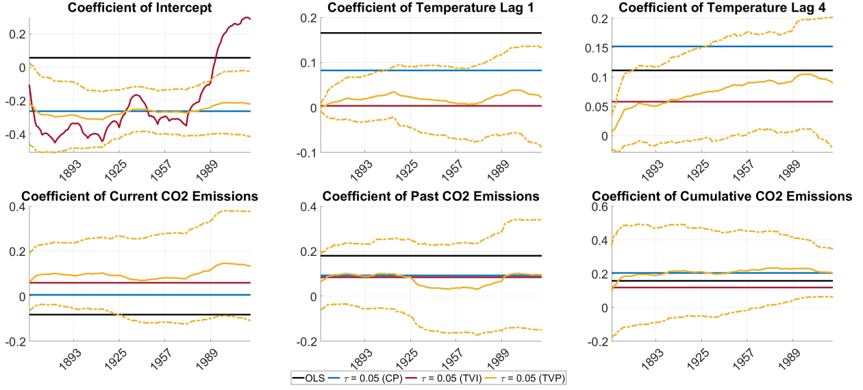
Figure 8: Posterior estimates of the benchmark model for the 5 th quantile, estimated by a constant parameter quantile regression, a time-varying intercept only alternative and a full time-varying parameter specification (including one standard deviation confidence bands), along with the OLS estimate.
