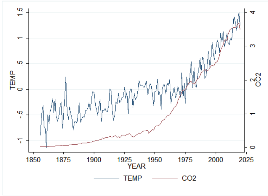
Figure 1: Temperatures and CO_2 emissions over the sample period.
