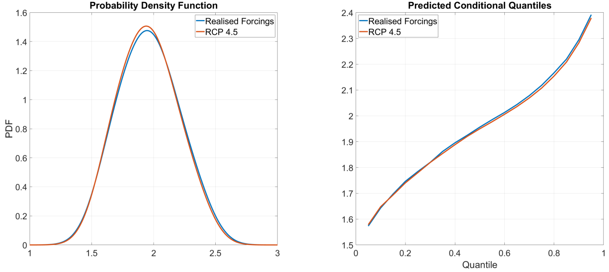
Figure 7: Predicted probability density function (left panel) and predicted conditional quantiles (right panel) for 2030 average global temperatures, given realized emissions and target emissions under RCP 4.5.
