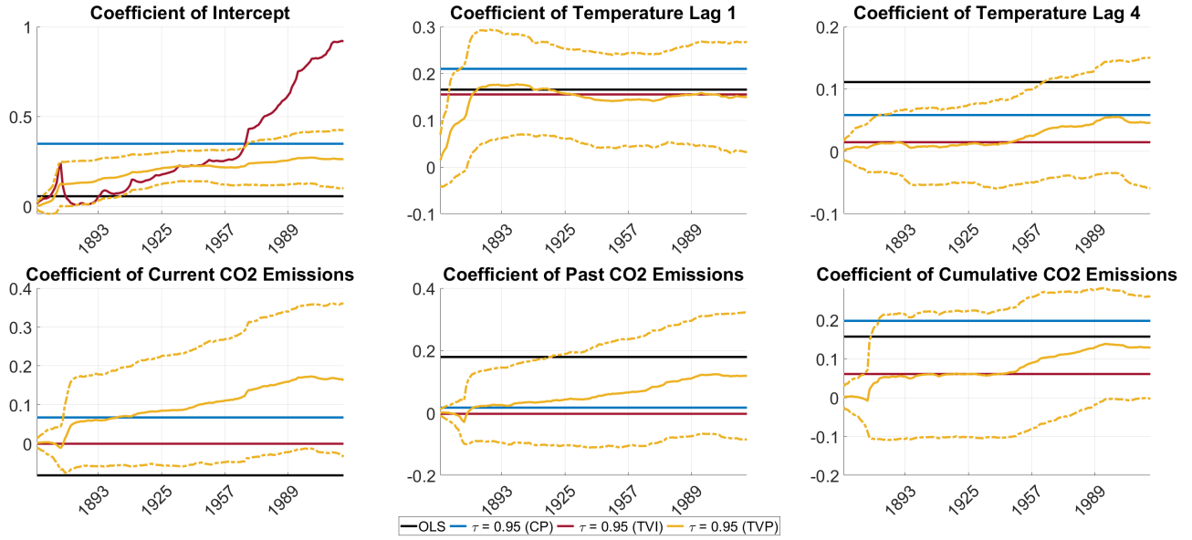
Figure 4: Posterior estimates of the benchmark model for the 95 th quantile, estimated by a constant parameter quantile regression, a time-varying intercept only alternative and a full time-varying parameter specification (including one standard deviation confidence bands), along with the OLS estimate.
