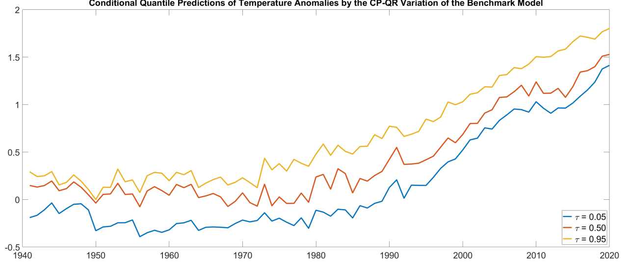
Figure 3: Conditional quantiles of temperature anomalies based on the CP-QR variation of the benchmark model.
