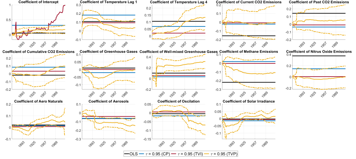
Figure 10: Posterior estimates of the model with all climate forcings for the 95 th quantile, estimated by a constant parameter quantile regression, a time-varying intercept only alternative and a full time-varying parameter specification (including one standard deviation confidence bands), along with the OLS estimate. 26
