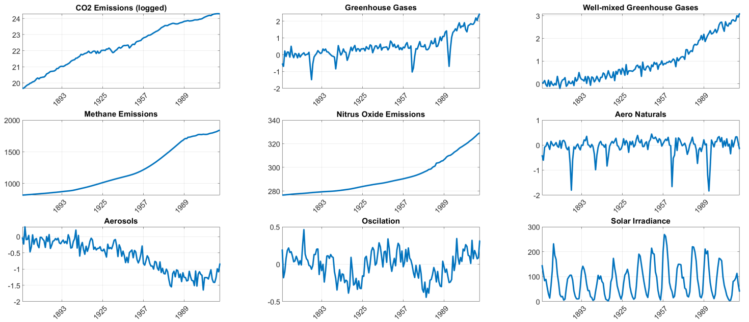
Figure 2: Climate forcings over the sample period.
