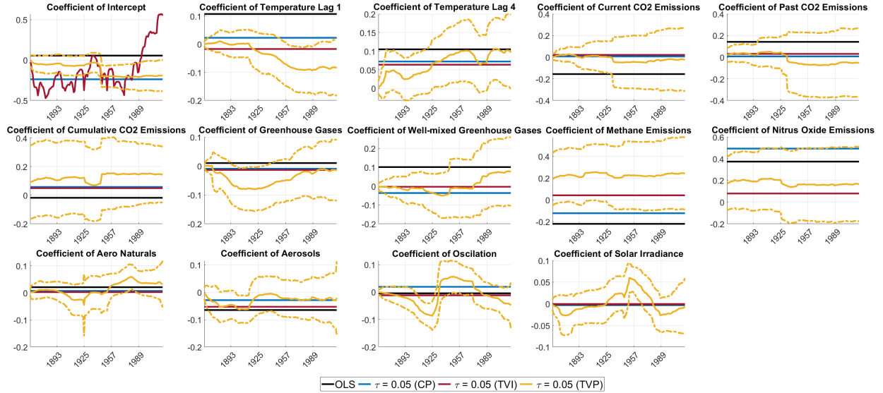
Figure 9: Posterior estimates of the model with all climate forcings for the 5 th quantile, estimated by a constant parameter quantile regression, a time-varying intercept only alternative and a full time-varying parameter specification (including one standard deviation confidence bands), along with the OLS estimate. 25
