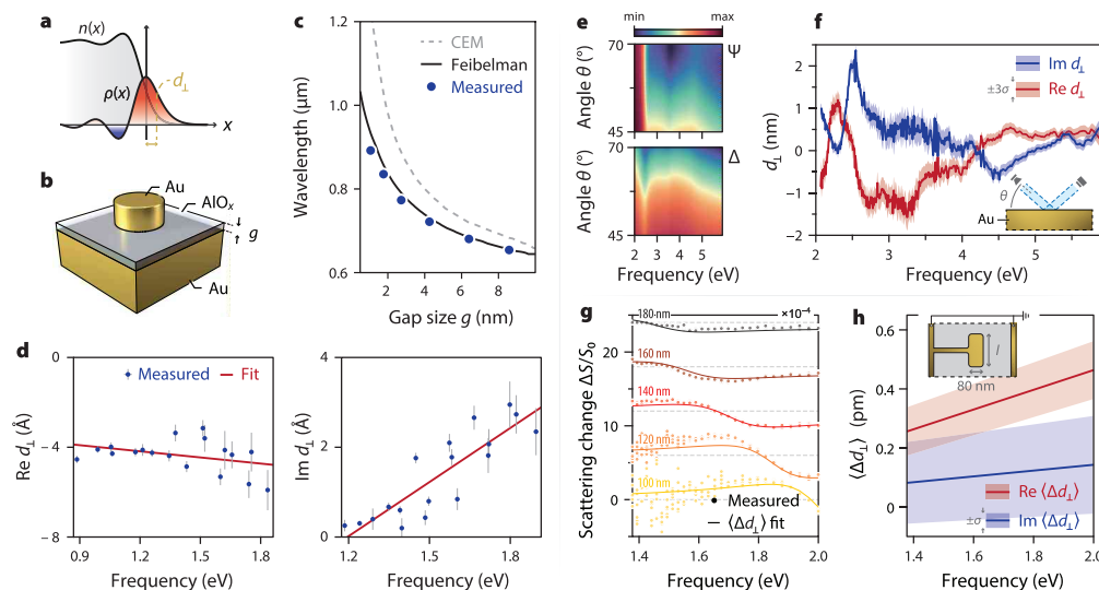
Fig. 16. Measuring Feibelman parameters. (a) The d_{\perp} and d_{\parallel} parameters are the frequency-dependent centroids of the induced charge \rho(x) (shown) and the normal derivative of the interface-tangential current \partial_x J_y(x) (not shown). Both \rho(x) and J_y(x) are induced quantities due to an incident plane wave, appearing as perturbations to the static equilibrium density n(x) . (b–d) Comparing observations of large deviations between CEM and experiments in gapped film-coupled nanodisks (b,c) with perturbation theory, Eq. (56), can enable experimental inference of the Feibelman parameters (d), here of d_{\perp} for a gold (Au) aluminum oxide ( \text{AlO}_x ) interface [258]. (e,f) The angle- ( \theta ) and frequency-dependent amplitude contrast \Psi and phase difference \Delta of the complex reflection ratio r_p/r_s = e^{i\Delta} \tan \Psi between p - and s -polarized light are conventionally used to obtain a material's permittivity by fitting to the classical Fresnel reflection coefficients r_{p,s} . By using the Feibelman-corrected reflection coefficients instead, sufficiently precise measurements of \Psi and \Delta can enable inference of the interface's Feibelman parameters (f), here of d_{\perp} at an Au(111)–air interface [313]. (g,h) An external gate voltage of 10 V, applied over an Au nanoresonator, leads to a frequency-dependent shift \Delta S of the nanoresonator's scattering signal, presented relative to its ungated signal S_0 (b). Measurements over different nanoresonator lengths l are labeled, shifted vertically, and differentiated by color. The shift of the scattering signal may be interpreted as due to a gate-tunable (interface-averaged) shift \langle \Delta d_{\perp} \rangle of the d_{\perp} -parameter at the Au–air interface (h), obtained by fitting to experimental data [236]. Inset in (g) schematically illustrates the nanoresonator, its dimensions, and gating configuration. Panels (a,c,d) adapted with permission from Ref. [258] (Copyright © 2019 Springer Nature).; (e,f) adapted from Ref. [313]; (g,h) adapted from Ref. [236] (American Association for the Advancement of Science, CC BY 4.0).
