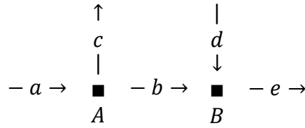
Figure 1. Traffic in the stochastic network
