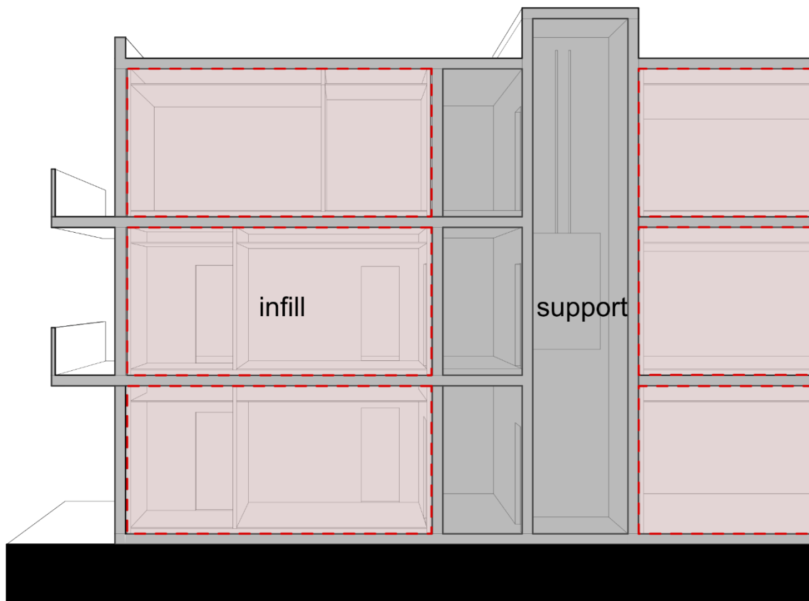
Figure 1: Support - the building systems that are common to all building owners, e.g., slabs, façade, roof, elevator shafts, floor landings...; and Infill - all building systems are part of a specific horizontal property, e.g., partition walls, dropped ceiling, raised floors, all services that specific to one apartment.
