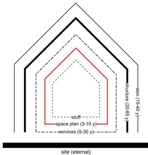
Figure 3: Shearing layers of change: a concept introduced by Francis Duffy (1990) for interiors and expanded by Steward Brand to the building level to describe the different rates at which different building subsystems change. Figure adapted from Brand (1994: 13) Reproduced with permission of Steward Brand
