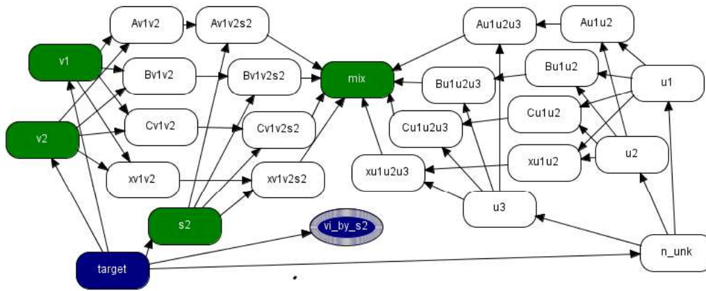
Figure 1 Marker network
