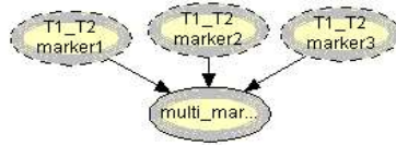
Figure 4 Accumulate network
