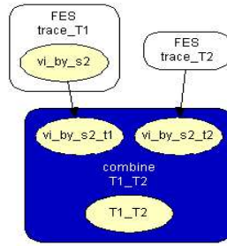
Figure 3 Combine_T1_T2 network
