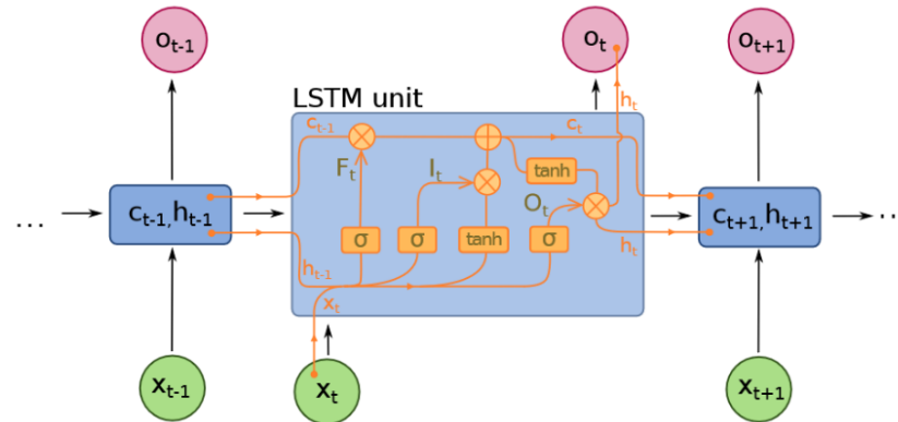
Figure 2. A LSTM network structure [60].
