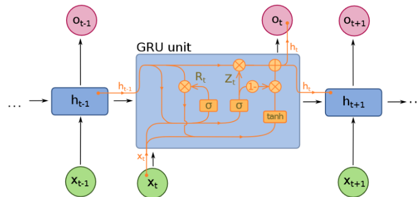
Figure 3. GRU network structure [64].
