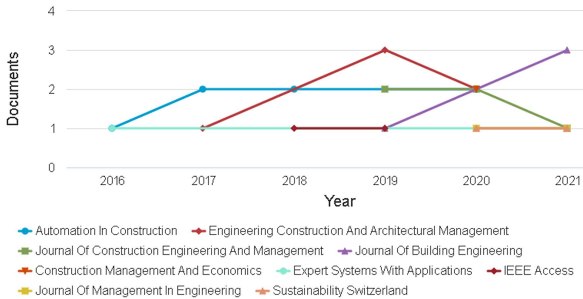
Figure 5 - Documents per year per source (Top 9 sources). Source: Scopus.
