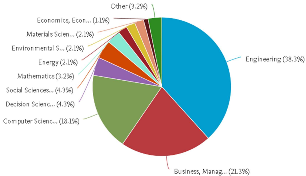
Figure 4 - Documents by subject area. Source: Scopus.
