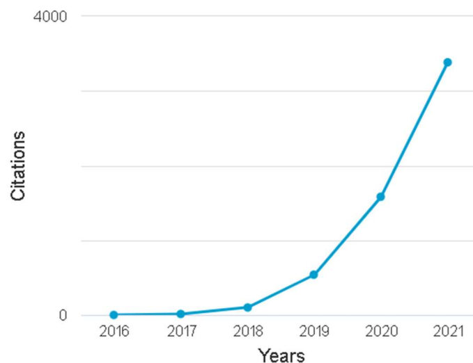
Figure 6 - Citations per year. Source: Scopus.
