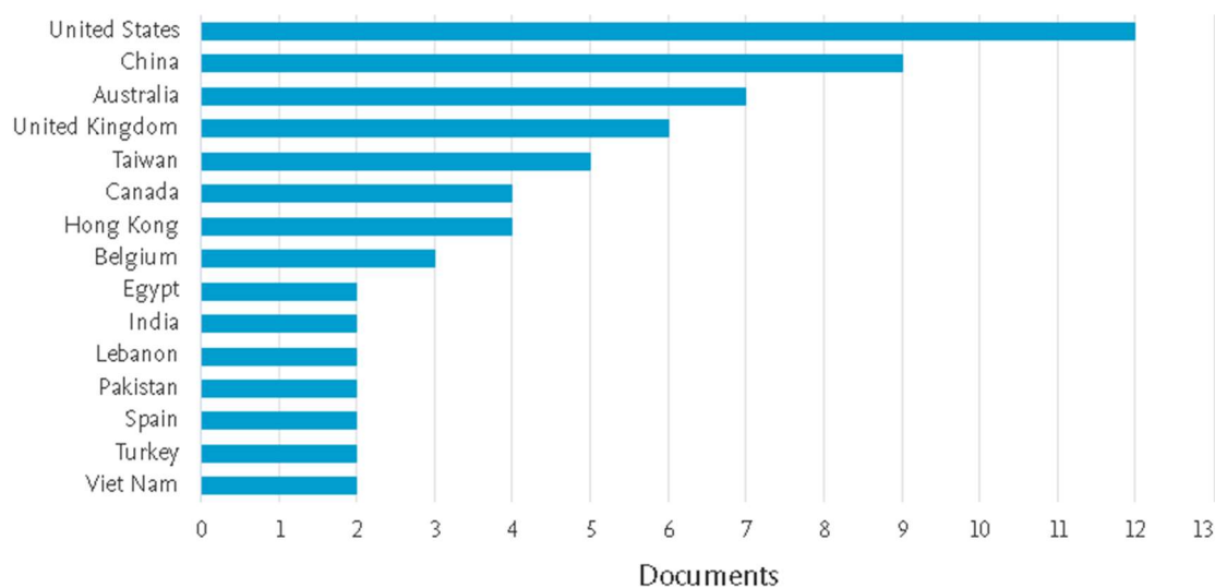
Figure 3 - Top 15 of the countries with more documents. Source: Scopus.
