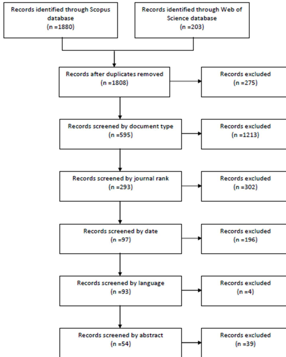
Figure 1 - Data selection process (PRISMA methodology). Source: Author.
