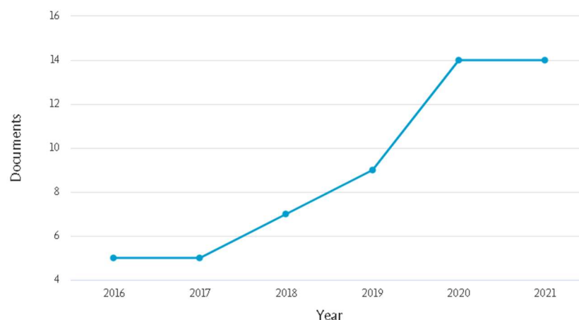
Figure 2 - Documents per year. Source: Scopus.
