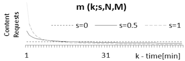
Figure 3. Theoretical curve of Zipf equation
