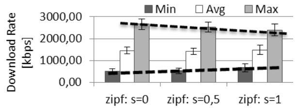
Figure 4. Download rate
