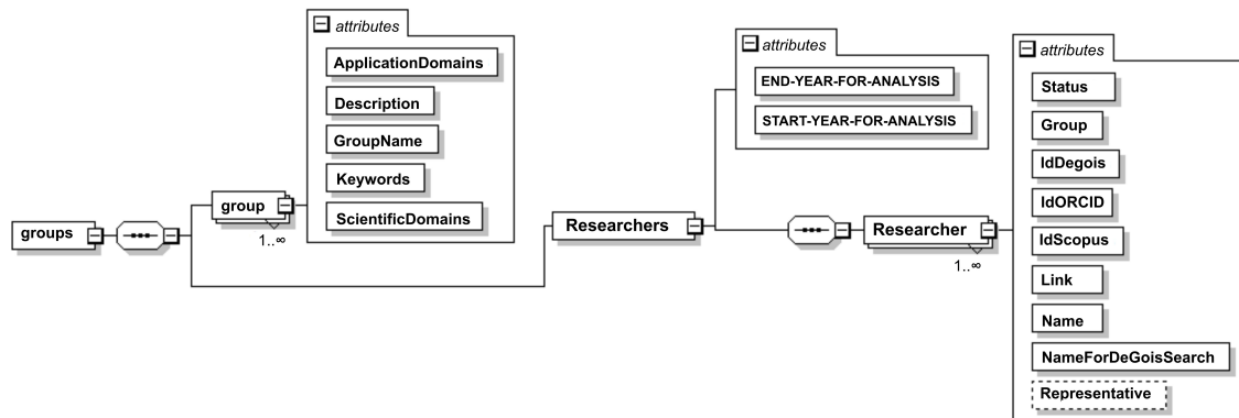
Figure 5. Researchers.xml Schema [20].
