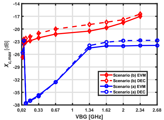
Figure 8: Tolerated crosstalk level as a function of the VBG considering the DEC (dashed lines) and EVM (solid lines) estimations.
