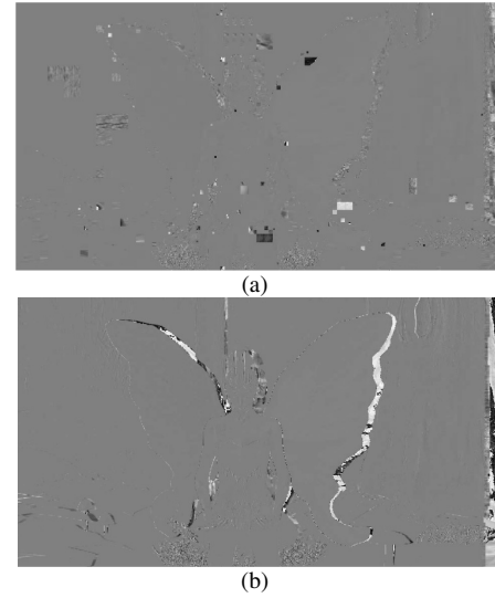
Figure 5 Residual luminance for the first inter coded right view using: (a) HEVC MVD ; and (b) MV direct-DV (Mode)
