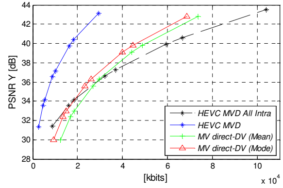
Figure 4 RD performance for the proposed MV direct-DV coding scheme
