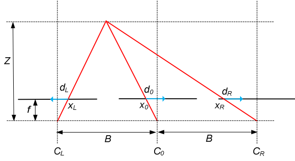
Figure 1 Disparity vector derivation considering a parallel camera geometry
