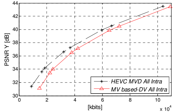
Figure 8 RD performance for the MV base-DV coding scheme considering an “All Intra” configuration
