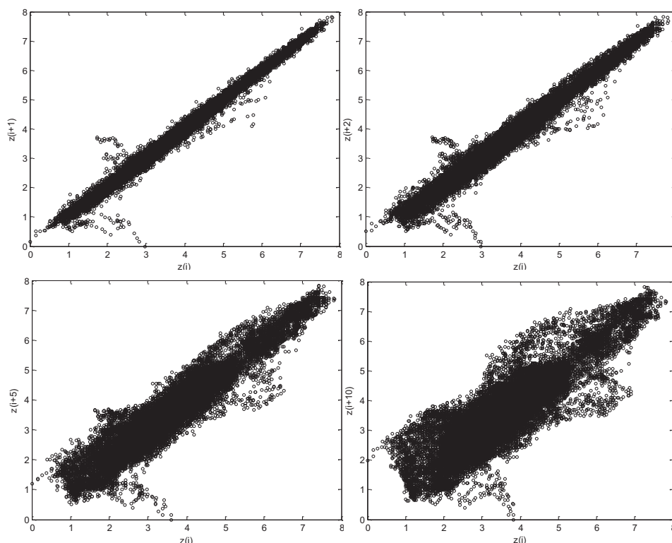
Fig. 6. Surface correlograms for distances ( lag ) of 0.5 ( i +1), 1.0 ( i +2), 2.5 (+5) and 5.0 mm ( i +10)
