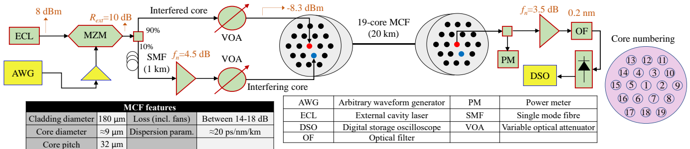
Fig. 1: Experimental setup employed to assess the influence of the skew-bit rate product on the photodetected OOK signal.
