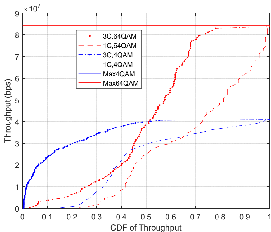
Figure 8. Throughput performance (bps) vs. CDF of throughput for UMa scenario with N_{tx} = 5N_u , N_f = 4 , N_{of} = 3 , N_s = 5 , N_u = 2 , N_{rx} = 5 , 64QAM (11.75 bpcu per user) and 4QAM (5.75 bpcu per user).
