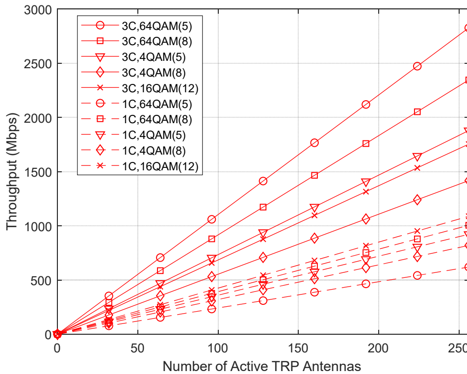
Figure 11. Throughput vs. number of active TRP antennas, for UMi scenario, N_{rx} = 5 , for two C-RAN cluster sizes, modulations and numbers of antennas per user, namely with N_{tx}/N_u = 5 , 64QAM(5) and 4QAM(5); with N_{tx}/N_u = 8 , 64QAM(8) and 4QAM(8); and with N_{tx}/N_u = 12 , 16QAM(12).
