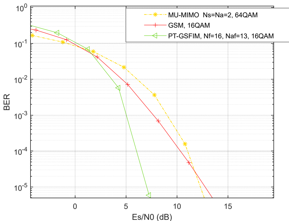
Figure 4. Comparison of BER performances of PT-GSFIM, GSM and conventional BD MU-MIMO, with N_u = 8 and SE = 12 bpcu.
