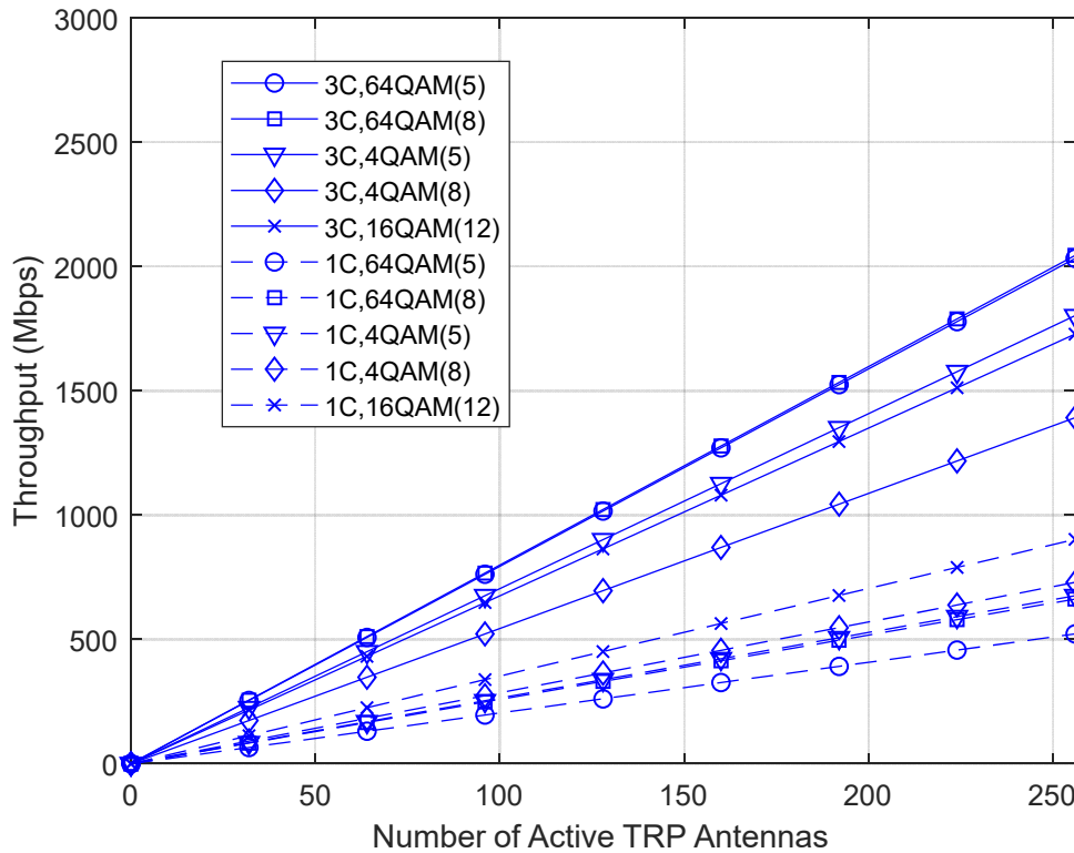
Figure 10. Throughput vs. number of active TRP antennas, for UMA scenario, N_{rx}=5 , for two C-RAN cluster sizes, modulations and numbers of antennas per user, namely with N_{tx}/N_u=5 , 64QAM(5) and 4QAM(5); with N_{tx}/N_u=8 , 64QAM(8) and 4QAM(8); and with N_{tx}/N_u=12 , 16QAM(12).
