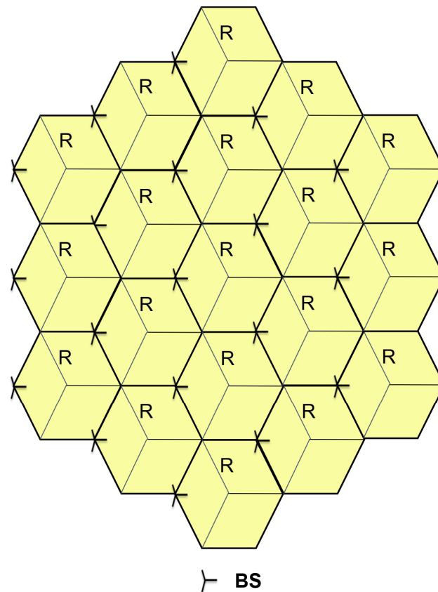
Figure 2. Urban micro scenario layout: Macro layer: ISD = 200\text{ m} = 3R ; Micro layer: 3 micro TRPs per macro TRPs.
