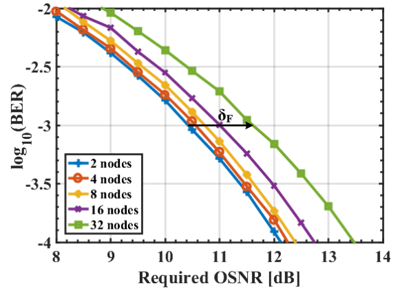
Fig. 7. BER as a function of the required OSNR for a 50-Gb/s NRZ QPSK signal that passes through a cascade of ROADM nodes.
