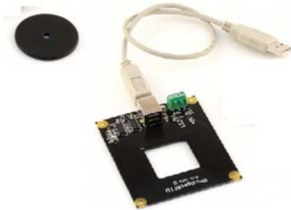
Fig. 4. LF RFID reader embedded in the box and LF tags embedded in the red and green color cubs for cubs 'identification.
