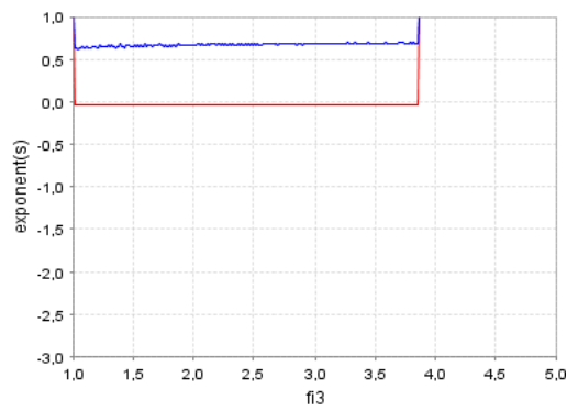
FIG. 50. model 3; Lyapunov exponents [ k_0 = 8; d_0 = 0.25; 1 \leq \phi_3 \leq 5; \phi_4 = 0.7; \text{iterations}=1000 ]
