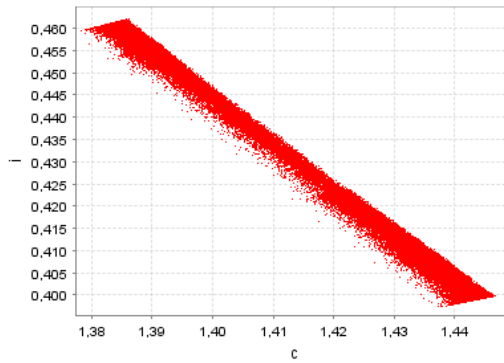
FIG. 30. model 2; attractor - variables c_t, i_t [ k_0 = 8; d_0 = 0.25; \phi_0 = 0.2; \phi_1 = 0.5; \phi_2 = 5; \text{transients}=1000; \text{iterations}=100,000 ]
