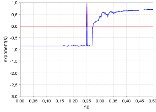
FIG. 22. model 1; Lyapunov exponents [ k_0 = 8 ; d_0 = 0.25 ; 0 \leq \phi_0 \leq 0.5 ; \phi_1 = 2.5 ; iterations=1000]
