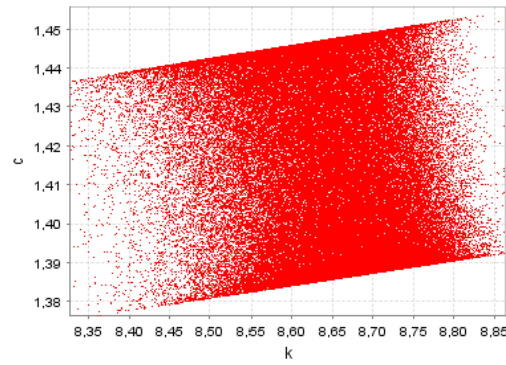
FIG. 47. model 3; attractor (k_t, c_t) [ k_0 = 8; d_0 = 0.25; \phi_3 = 2.5; \phi_4 = 0.7 ; transients=1000; iterations=100,000]
