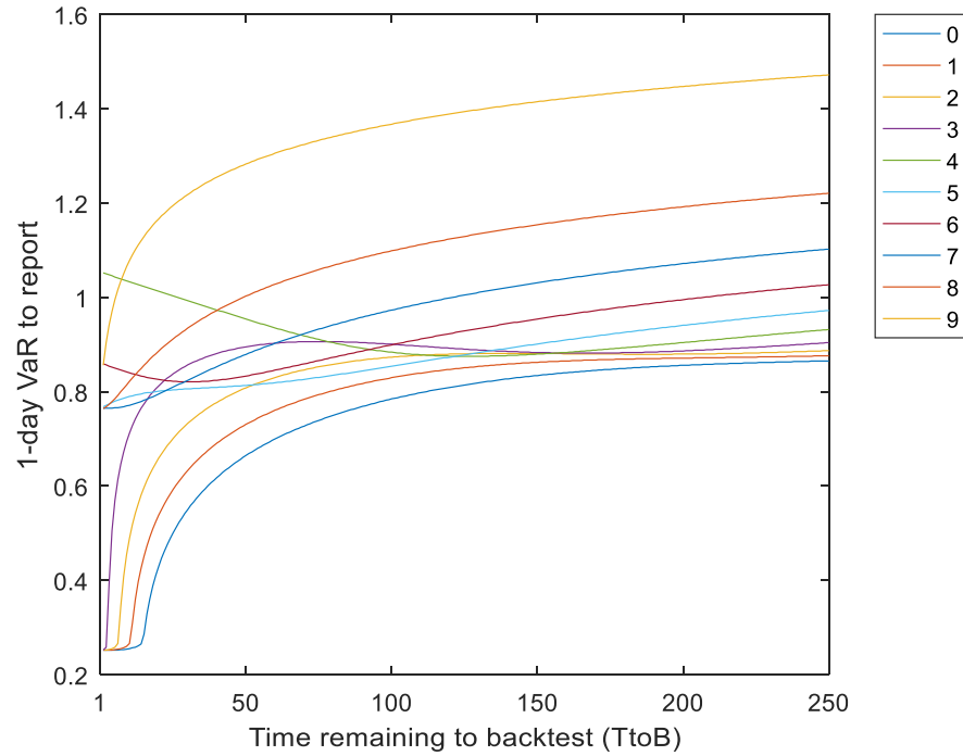
Figure 27 – Optimal policy function for all the number of exceedances when the multiplier k is equal to 4.
