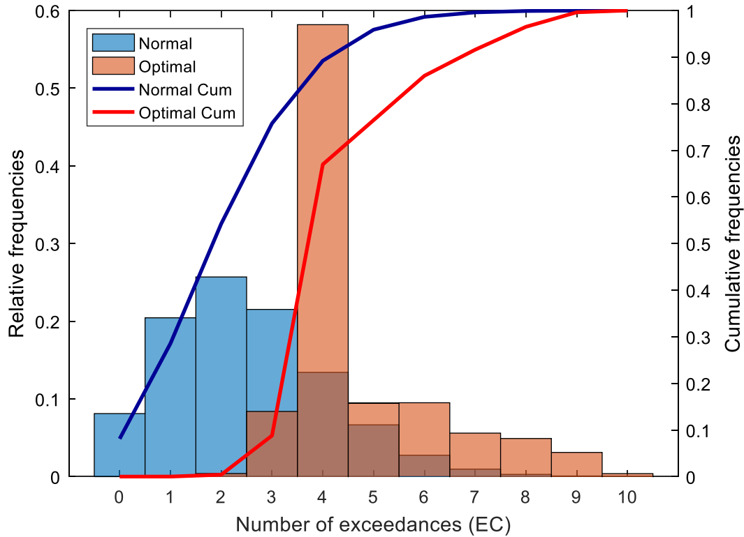
Figure 6 – Distribution of the EC variable, in the end of the period, across the various simulations, and the respective cumulative frequencies (right axis).
