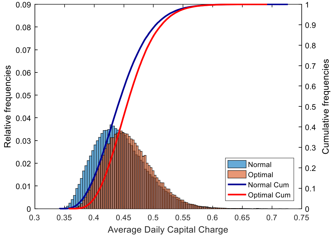
Figure 12 – Distribution of the average daily capital charge across simulations, and the respective cumulative frequencies (right axis), for a 20% undervaluation level.
