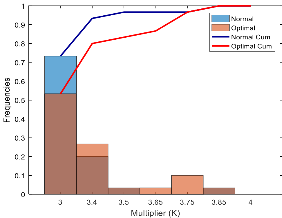
Figure 20 – Distribution of the multiplier (K) variable, for the portfolio simulation.
