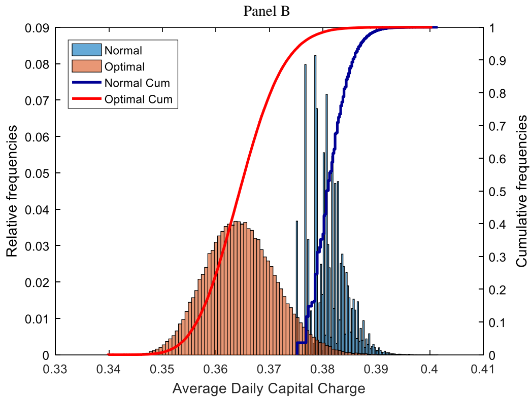
Figure 15 – Distribution of the average daily capital charge in each simulation and the respective cumulative frequencies (right axis), for the simplified model simulation (Panel A) and the normal simulation (Panel B).
