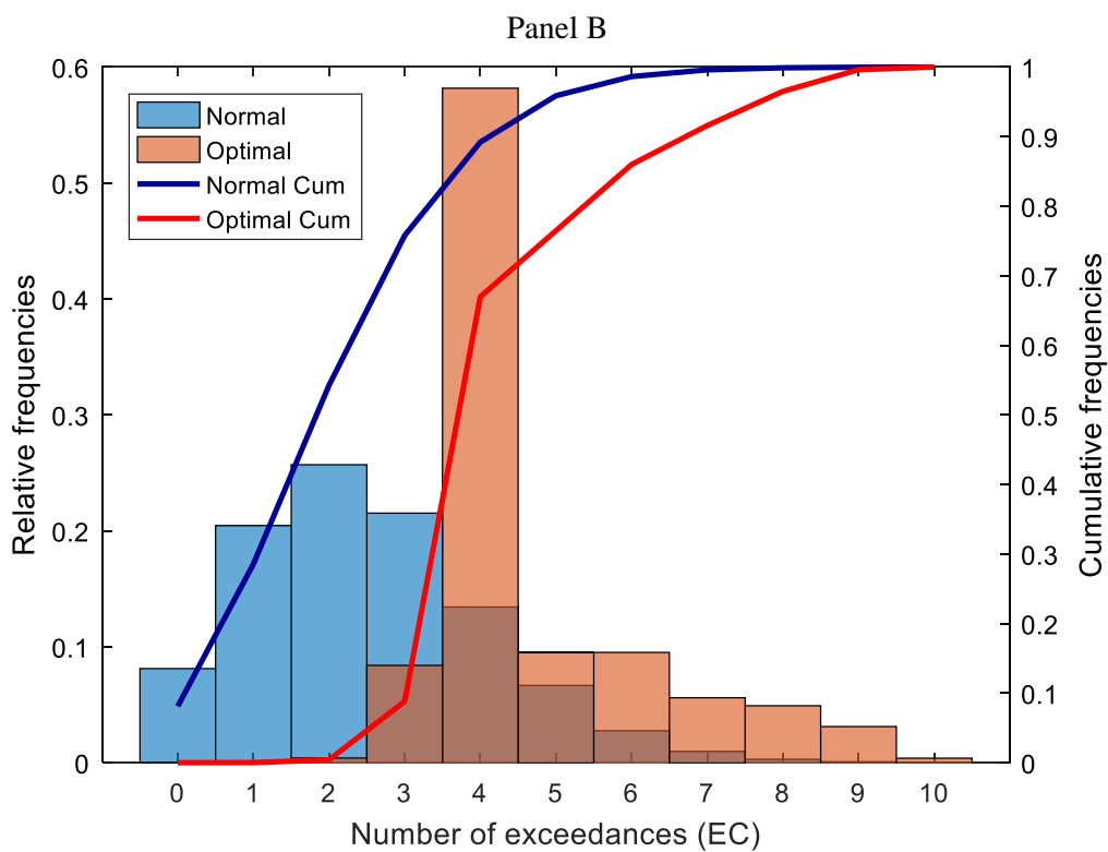
Figure 16 – Distribution of the EC variable, in the end of the period, across the various simulations, and the respective cumulative frequencies (right axis), for the simplified model simulation (Panel A) and the normal simulation (Panel B).
