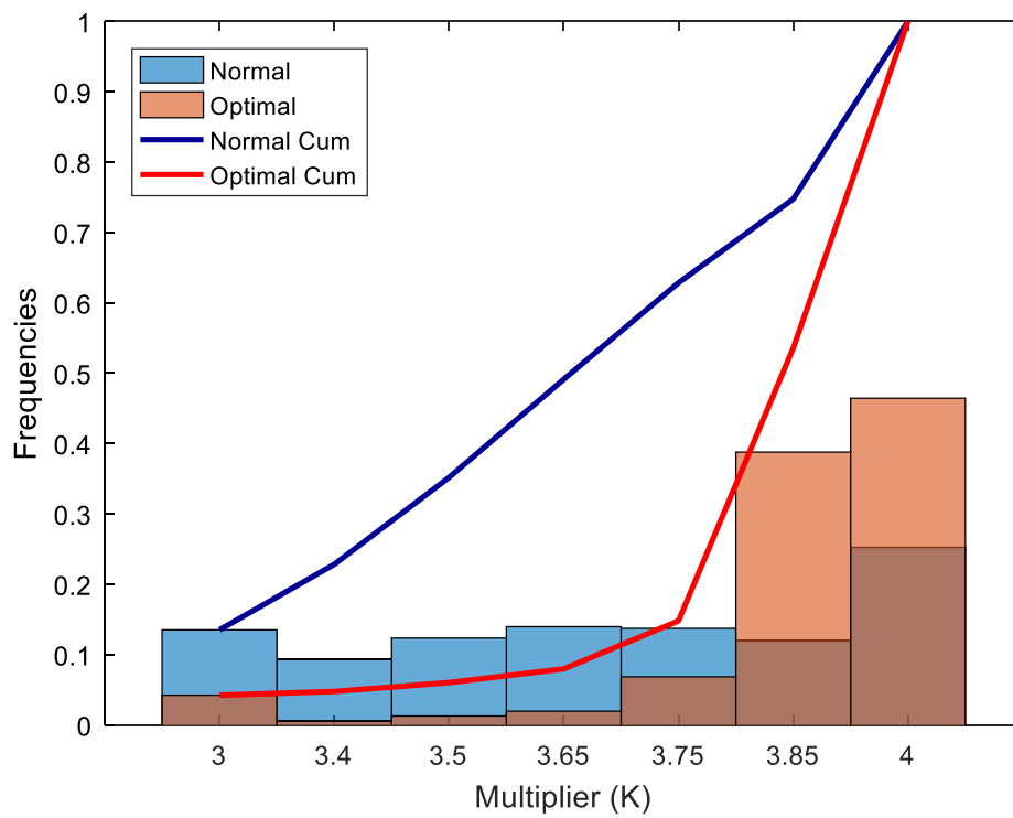
Figure 14 – Distribution of the multiplier k variable across the various simulations and the respective cumulative frequencies, for a 20% undervaluation level.
