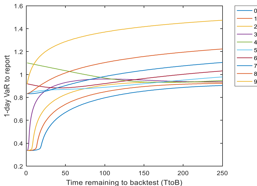
Figure 21 – Optimal policy function for all the number of exceedances when the multiplier k is equal to 3.
