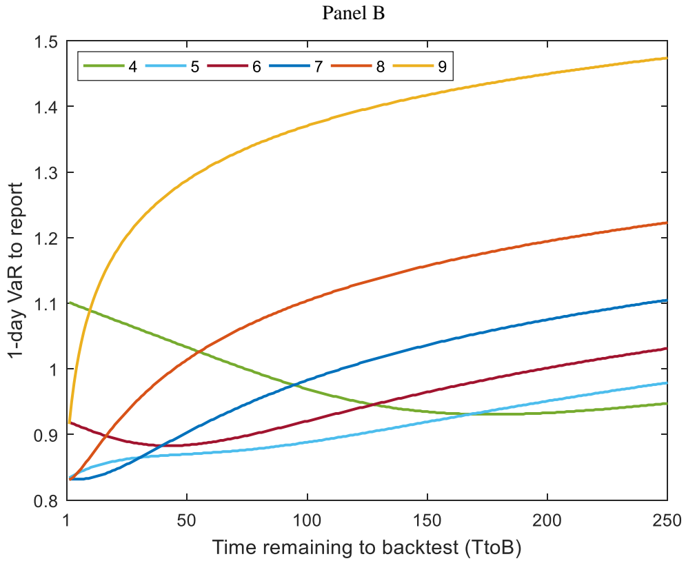
Figure 1 – Optimal Policy Function for a number of exceedances of 0 to 3 (Panel A) and 4 to 9 (Panel B) when the multiplier k is equal to 3.
